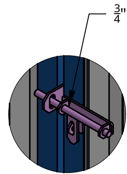
DETAIL A Slide Latch (Lock by Others)
