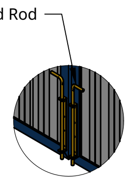
DETAIL B Cane Bolt (Lock by Others)
